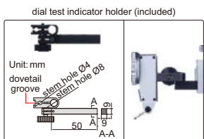
dial test indicator holder (included)
