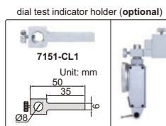
dial test indicator holder (optional)
