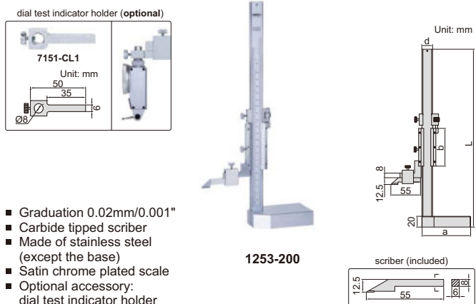
dial test indicator holder (optional)
