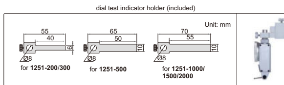
dial test indicator holder (included)
