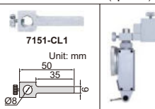
dial test indicator holder (optional)
